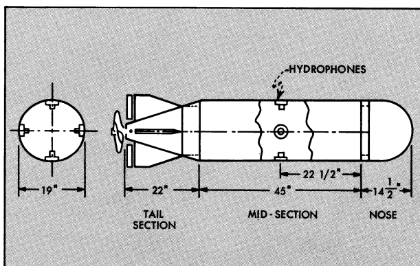
Sketch of acoustic torpedo developed and produced during World War II. It was credited with sinking 37 U-boats and seriously damaging 18 others.
