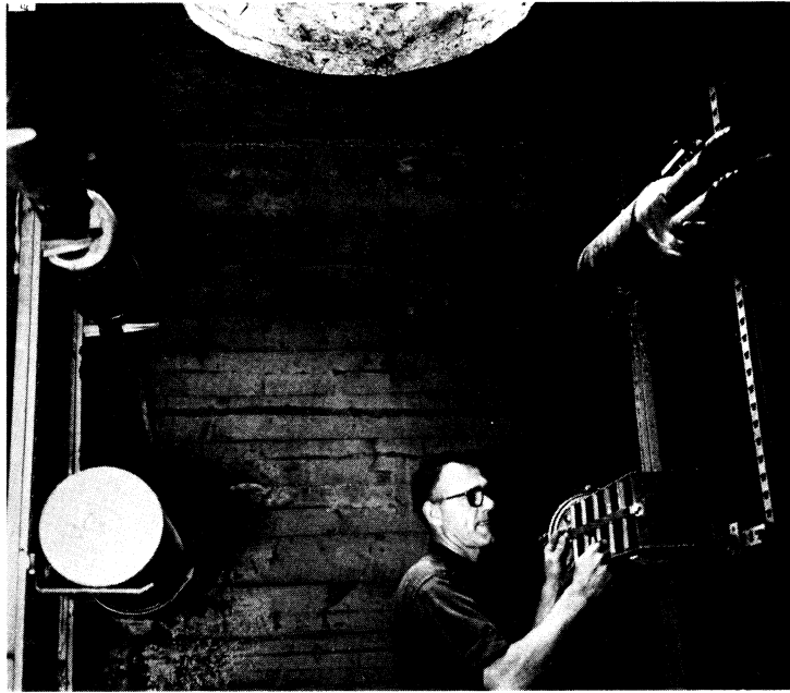
A splicer completing installation of T1 repeaters in an apparatus case in a typical manhole. The T1 signals are regenerated at 6000-foot intervals along the route. Today, with some 2½ million circuits in place, T1 supplies almost all the carrier growth in typical metropolitan areas.
