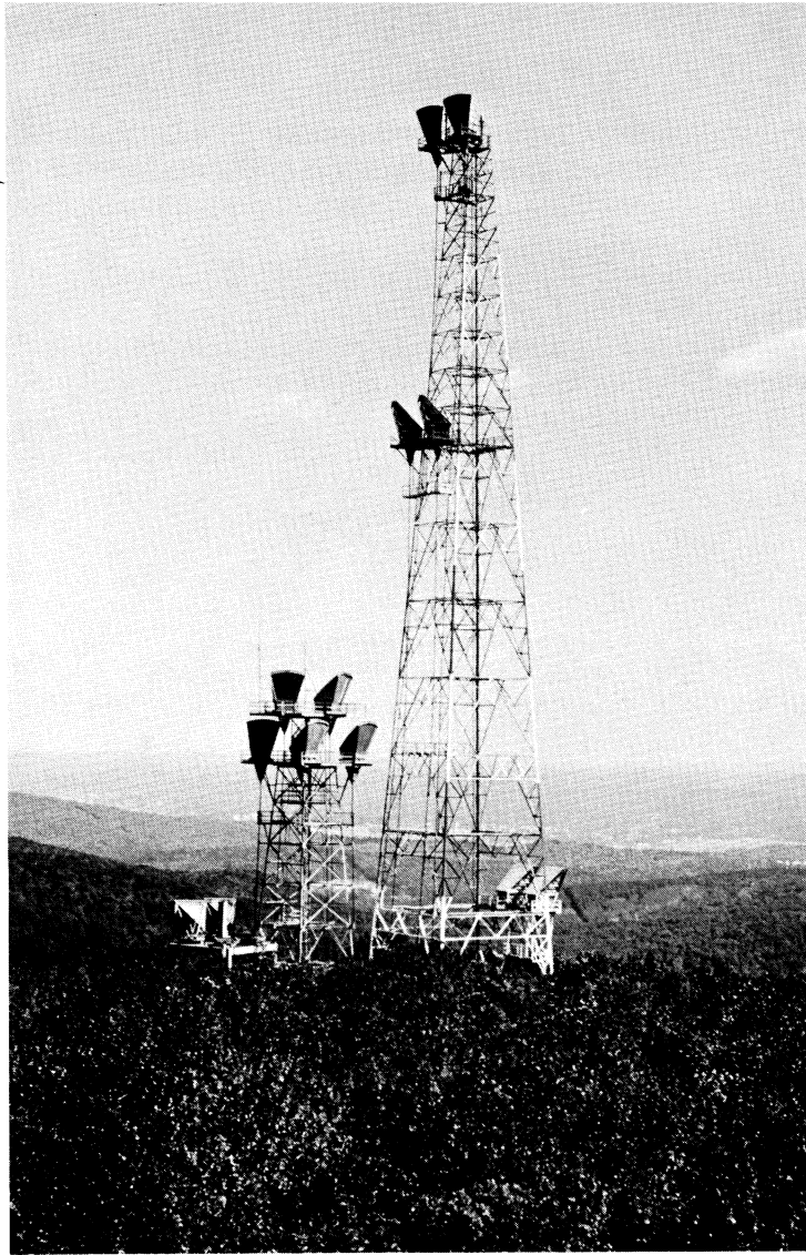
Present microwave station at Jackie Jones, New York—one of the original sites for the trial microwave radio relay system in 1947. The original trial antenna is just visible over the treetops at left of the towers.
