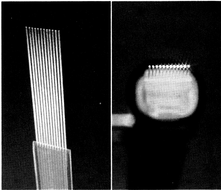
Optical fibers—drawn from specially prepared low-loss glass “preforms” and assembled as orderly cable strands in a protective sheath—will be the heart of future fiberoptic transmission systems. The width of a ribbon consisting of several fibers is typically about \frac{1}{8} inch.
