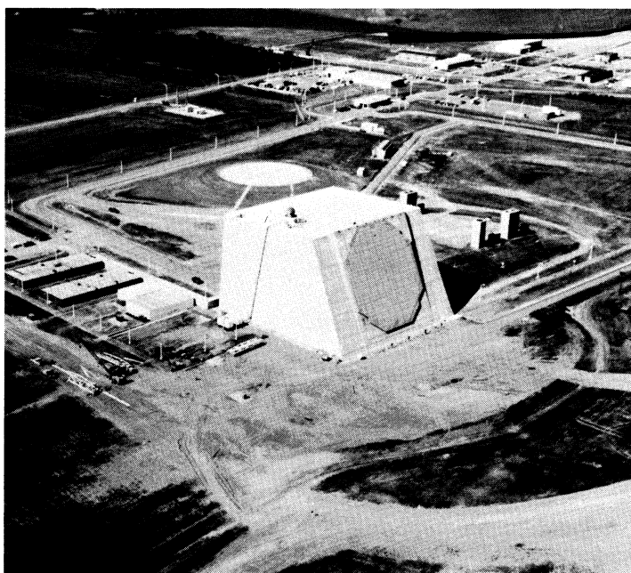
Grand Forks, N. D., site of the Safeguard Ballistic Missile Defense System (top), and view of the Perimeter Acquisition Radar (bottom) at Grand Forks.
