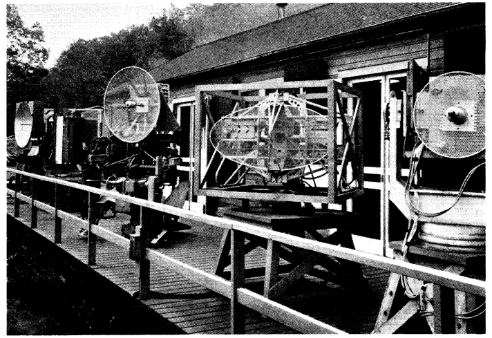
From this Atlantic Highlands, N. J., cottage on a bluff overlooking the Ambrose Channel, engineers from Bell Laboratories successfully tested the first radar system that was specifically designed to plot ship movements at night.
