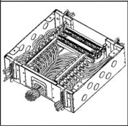
Figure 138b M32 CCP Zone Wiring Box
