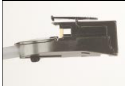
Figure 53 110 4-Pair GS XL Patch Cord
