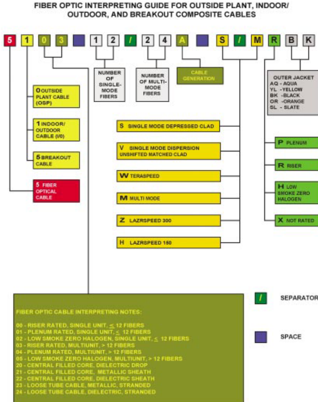
Figure 47 Marketing OSPI-O and B-O Composite Cables
