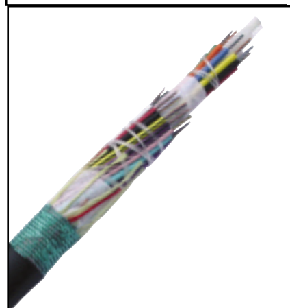
Figure 43 Stranded Loose Tube Metallic Cable
