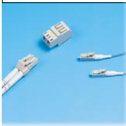
Figure 153 P1001A LC Connectors (right), Duplex MM LC Patch Cord (left) and C1001B-2 Adapter (center)
