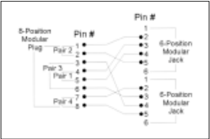
Figure 172 400E Pinout
