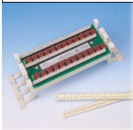
Figure 185 110RA2-12 ISDN Terminating Resistor Block
