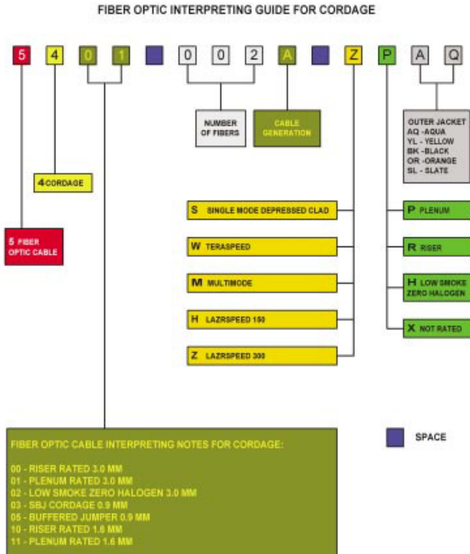
Figure 49 Marketing Cordage
