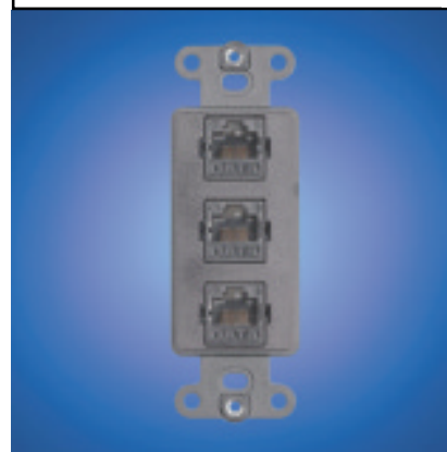
Figure 131 M108FR3 Decorative Frame
