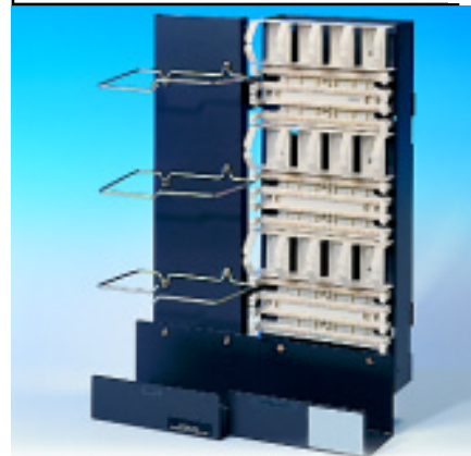
Figure 75 110PB2-300FT Patch Panel and 188D3 Backboard
