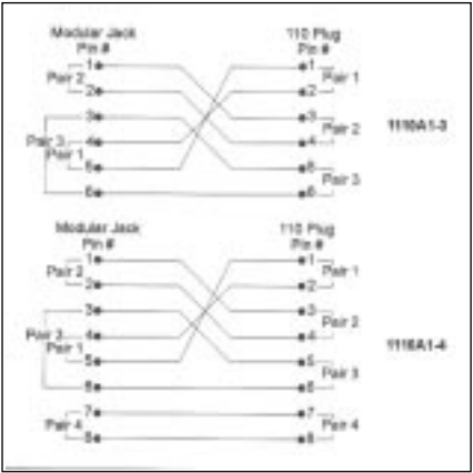
Figure 163 1110A1-3 and 1110A1-4 Pinout
