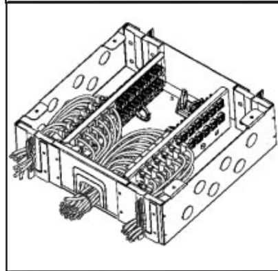
Figure 138c M48 CCP Zone Wiring Box
