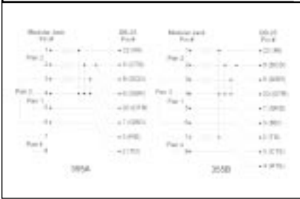
Figure 167 355 Pinout
