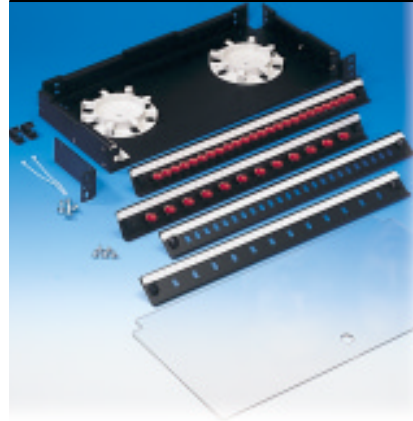
Figure 113 600A1 Shelf, 24 ST-EW, 12 ST-EW, 24 ST & 12 ST Panels, 183U1 Cover
