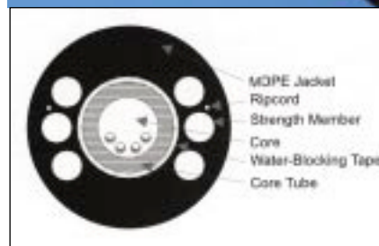
Figure 34 Dielectric Cable Cross Section
