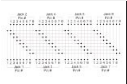
Figure 174 367A Pinout
