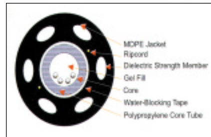
Figure 40 Cross Section
