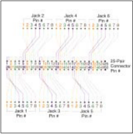
Figure 165 258A Pinout
